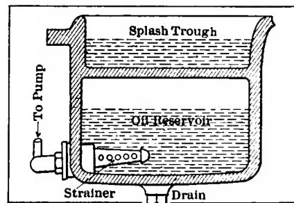
Fig. 3—Cunningham model H crankcase showing lead to pump
